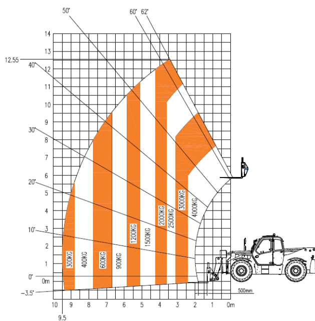
Without stabilizers, with chassis leveling
