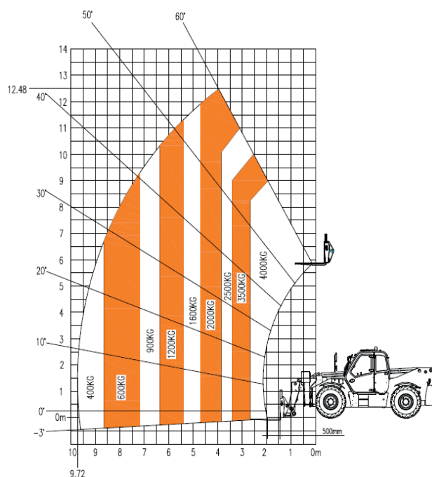
Without stabilizers, with chassis leveling
